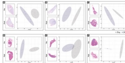
Figure 3: PCA 2D scores plots of lipids in tumor regions from biopsies pre- and post-treatment (B, mucosal and B-F, cutaneous melanoma). ROI were selected by high-magnification analysis of viable tumor regions of H&E-stained sections following DESI-MSI.
