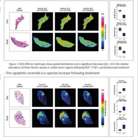
Figure 7: DESI-MSI on heparins show spatial distribution and a significant decrease ( p < .5 ) in the relative abundance of three HexCer species in viable tumor regions following NUC-7738 + pembrolizumab treatment
