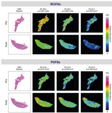
Figure 6: DESI-MSI on heparins show spatial distribution and a decrease in the relative abundance of three MUFA species and increase in three PUFA species in viable tumor regions following NUC-7738 + pembrolizumab treatment
